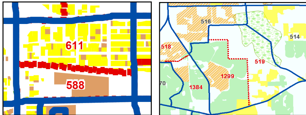
Figure 3.10 Delineating TAZs Based on Clusters of Similar Land Uses
